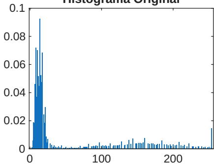
Histograma Original
